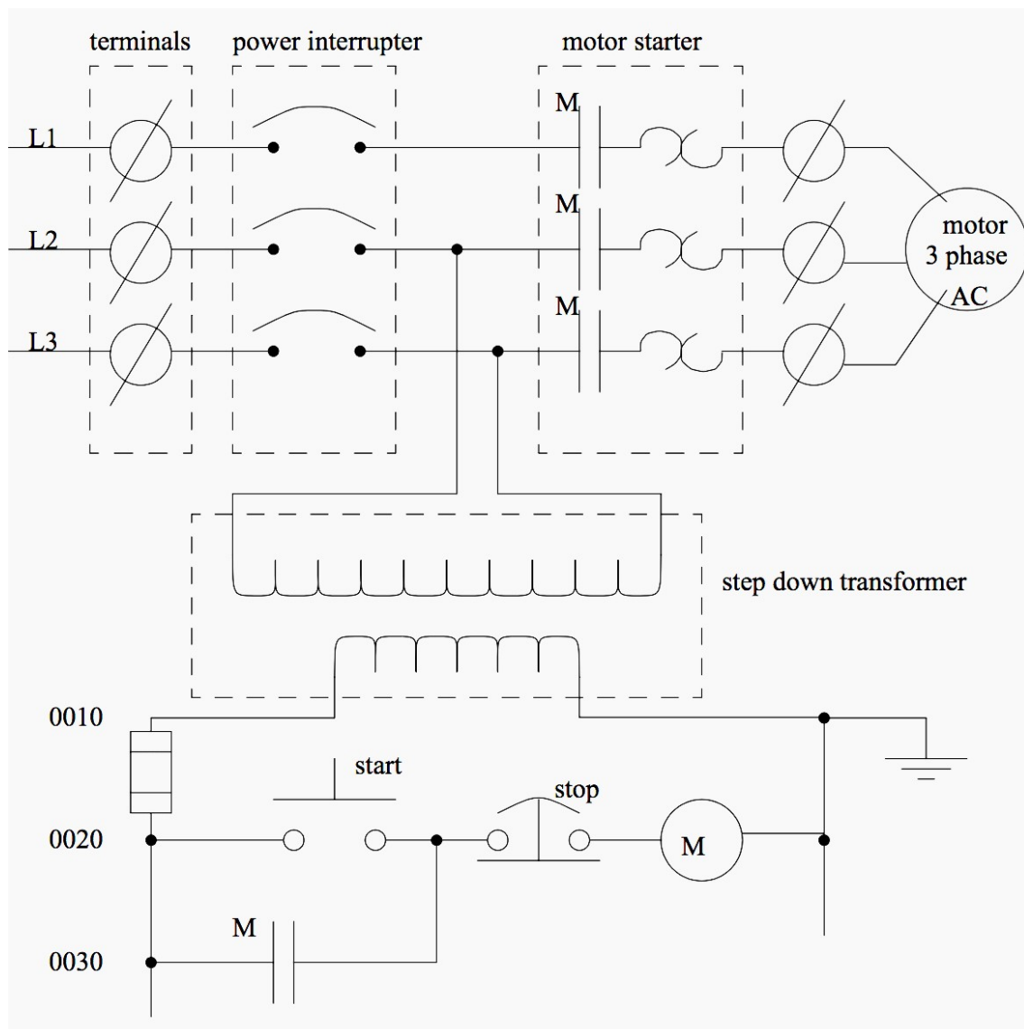
Figure 1 – A Motor Controller Schematic
